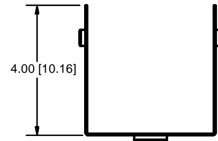
END VIEW
