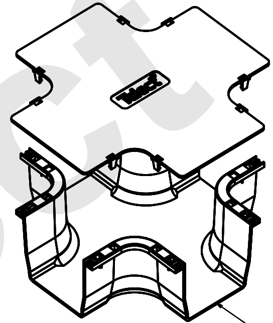
ISOMETRIC VIEW
